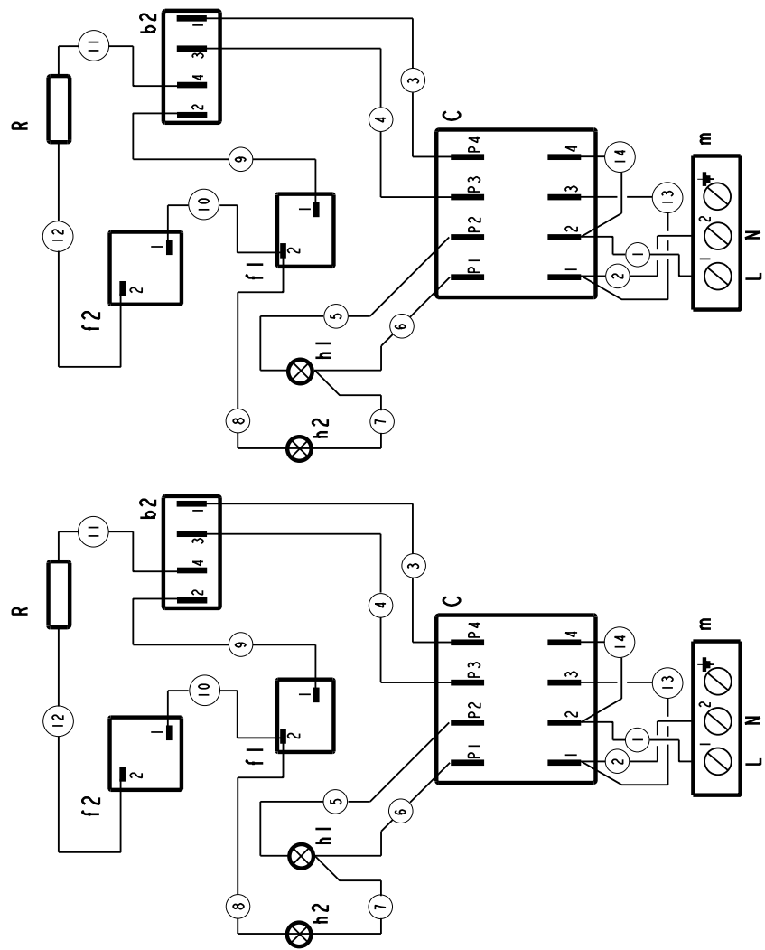
5415.101.00 Mod. 1 M SCHEMA ELETTRICO WIRING DIAGRAM V. 230/I
