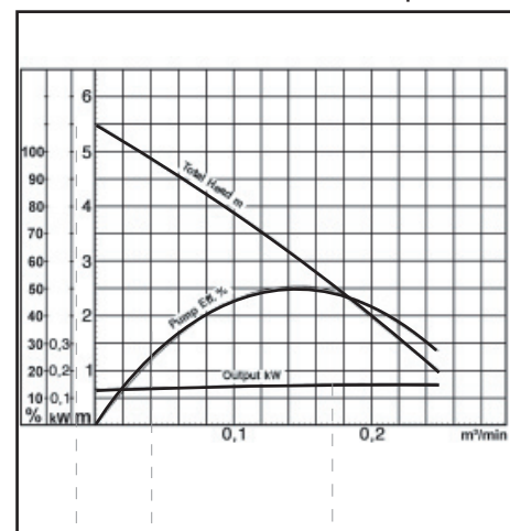
Total Head m Pump Eff. % Output kW
