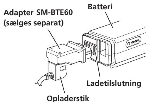
< BT-E6000/BT-E6001 >
