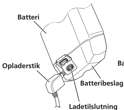
<BT-E6010>
