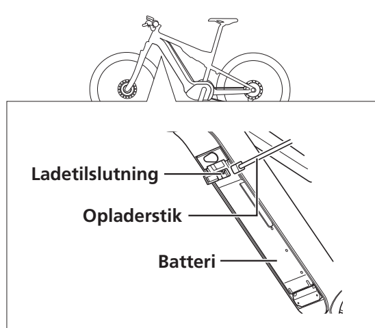
<BT-E8020>
