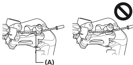
(A) Rille
