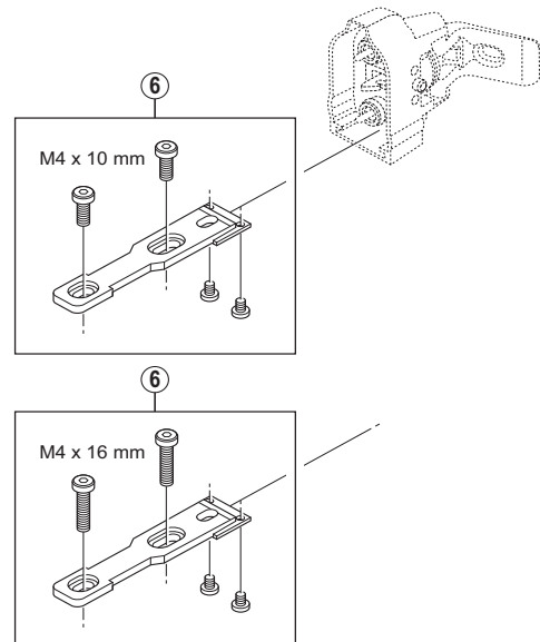
External / Internal type: Short size battery mount
