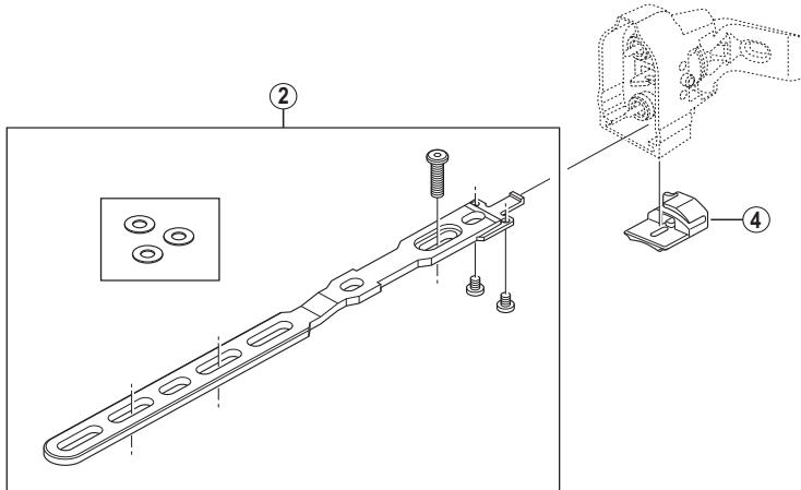
External type: Long size battery mount
