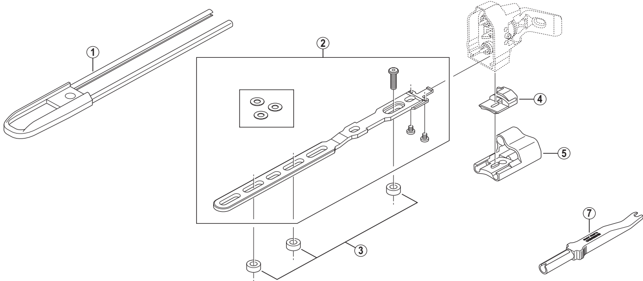
Internal type: Long size battery mount
