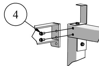
Detail S
