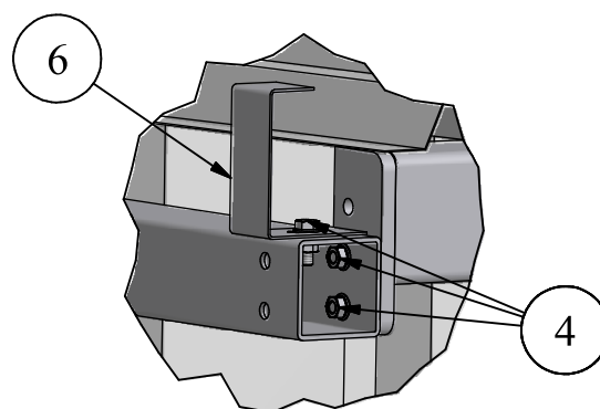
Detail K
