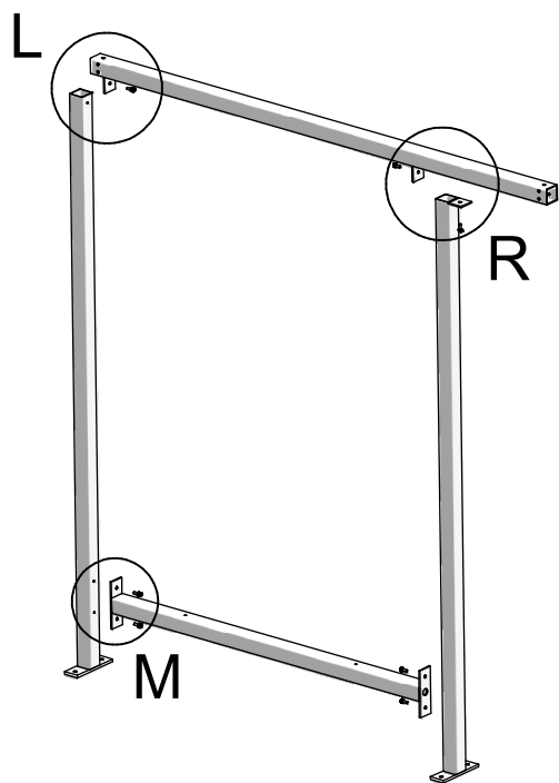
Detail M
