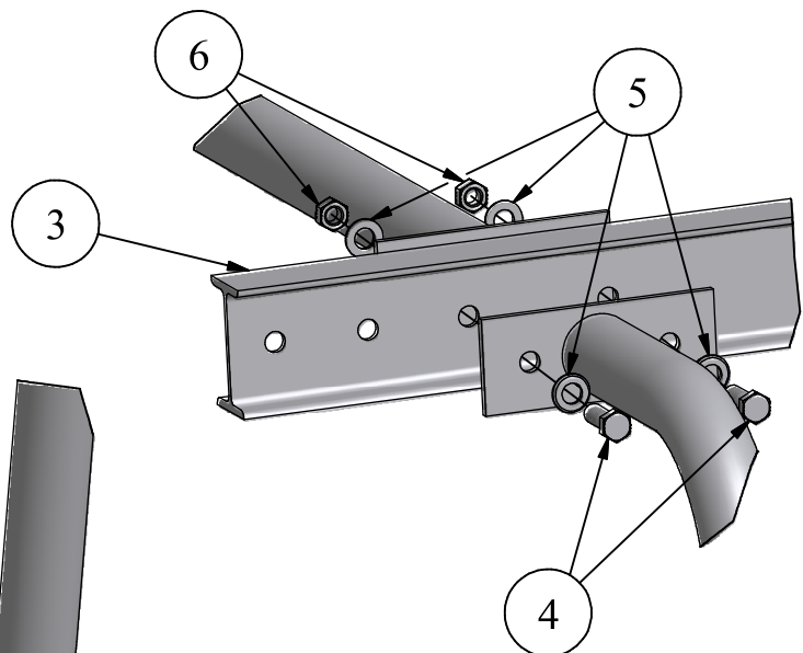
Detail B
